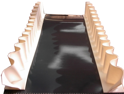
Flexible Borderflex Sidewalling for high product containment with flexibility around head and tail rollers
