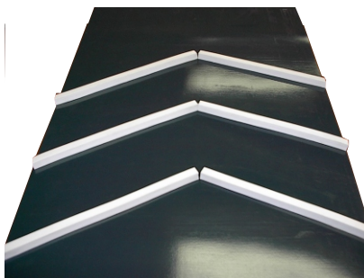
Herringbone profiles top side for product conveying and support on return rollers
