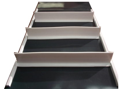
Longitudinal profile top side with cross cleats for high volume incline conveying and gooseneck conveyors where hold down rollers are utilised.
