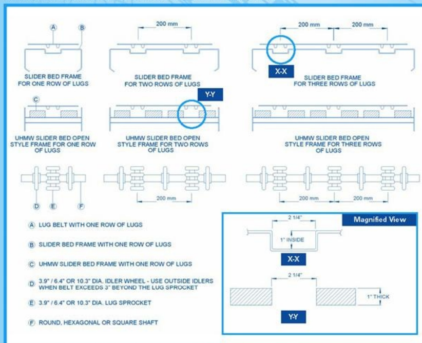
Typical Cog-Veyor bed showing drive lug arrangement and UHMW support strips
