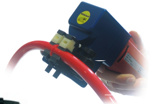
BEHA Patented RS 02 Friction Welder
