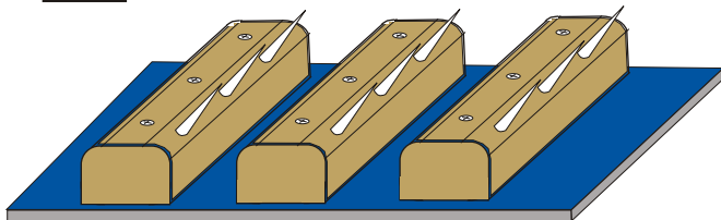
Inner slats on a P.V.C. belt
